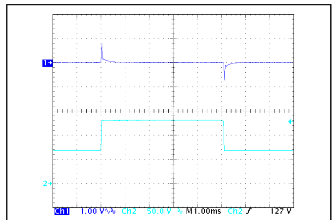
Figure 6: Output voltage response to step-change in input voltage (500 V/ms). Load cap: 100 \mu\text{F} , electrolytic output capacitance. Ch 1: Vout (1 V/div), Ch 2: Vin (50 V/div).
